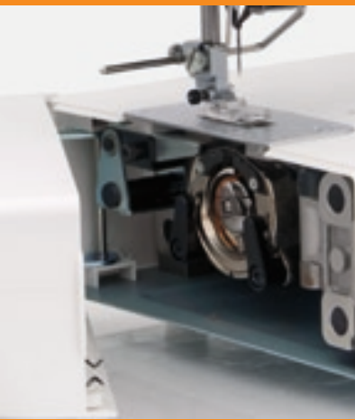
robustes CB-Greifer-System
